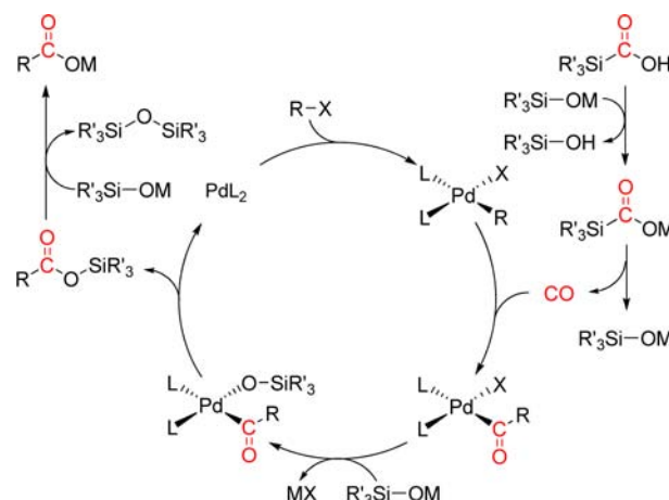
Scheme 5. Proposed Mechanism
